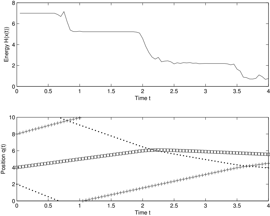
Figure 2: Plots of H(x(t)) and q_i(t) for initial data (2, 4, 8, -3, 1, 2) . Parameter values L = 10 , \gamma = \sigma = 1 , a_{ij} = 0 , r_c = 1 , and W^D defined by (1.2).
