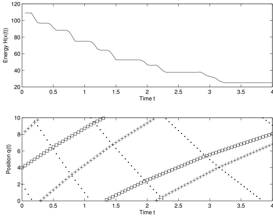
Figure 3: Plots of H(x(t)) and q_i(t) for initial data (2, 4, 8, -12, 5, 7) and parameters as in Figure 2.
