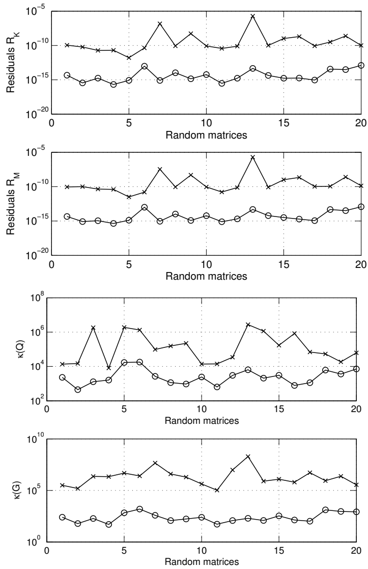
Figure 1. Residuals and condition numbers for 20 random matrices. Results from trd-L are marked with 'x' and results from trd-LH are marked with 'o'.
