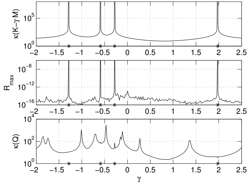
Figure 2. Influence of \gamma on \kappa(K - \gamma M) , \mathcal{R}_{\max} = \max(\mathcal{R}_K, \mathcal{R}_M) and \kappa(Q) for a 6 \times 6 random pair of symmetric matrices (K, M) .
