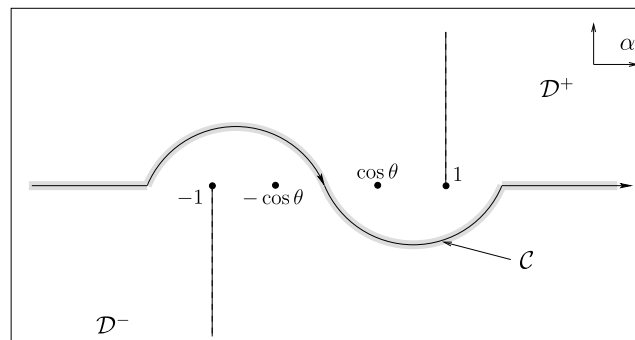
Fig. 2. The shaded area is the common strip of analyticity. Strip of analyticity for the integration path.
