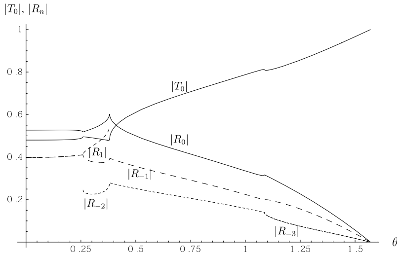
Fig. 10. |T_0|, |R_n| against \theta when a = 2.5 .
