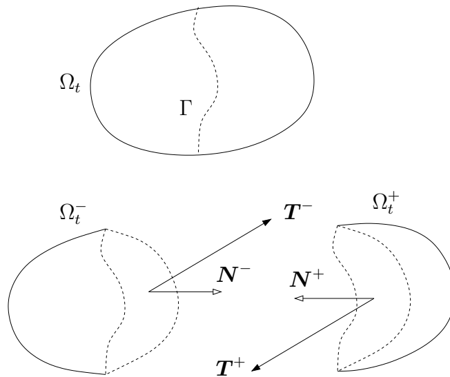
Figure 3.1: A region of a continuum \Omega_t is divided by a nominal internal surface \Gamma into the region \Omega_t^+ and \Omega_t^- . A outer unit normal can be defined for \Omega_t^+ and \Omega_t^- , say \mathbf{N}^+ and \mathbf{N}^- respectively. On \Gamma , \mathbf{N}^+ = -\mathbf{N}^- and the associated stress vectors, \mathbf{T}^+ and \mathbf{T}^- are also equal and opposite.
